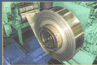
Skin Passing : Annealed coils are given skinpass-reduction of 0.50-2% to achieve desired surface finish-Dull/ Matt or Bright. Other metallurgical properties are achieved & Flatness of the strip is also improved.
