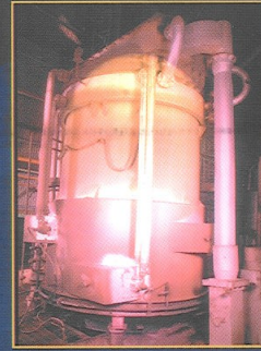
Annealing : As most of the applications demand Soft material the rolled coils are annealed in Bell type furnace equipped with inert atmosphere of N 2 and Hydrogen.
