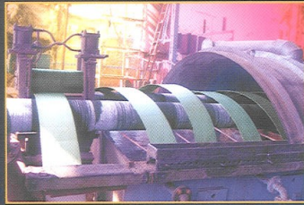
Spiral Pickling : Hot Rolled coils are pickled in Acid medium to remove scales and rust.
